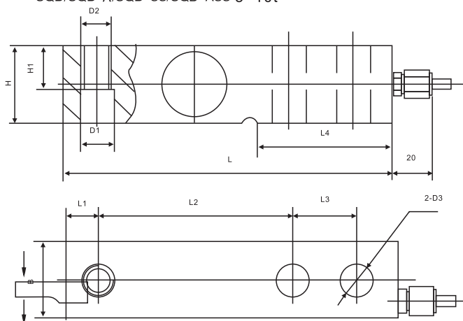
SQB/SQB-A/SQB-SS/SQB-ASS 3~10t
